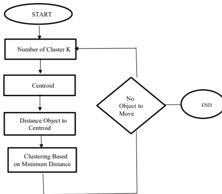
Fig.1. Flow Chart of K-Means Clustering Algorithm.
